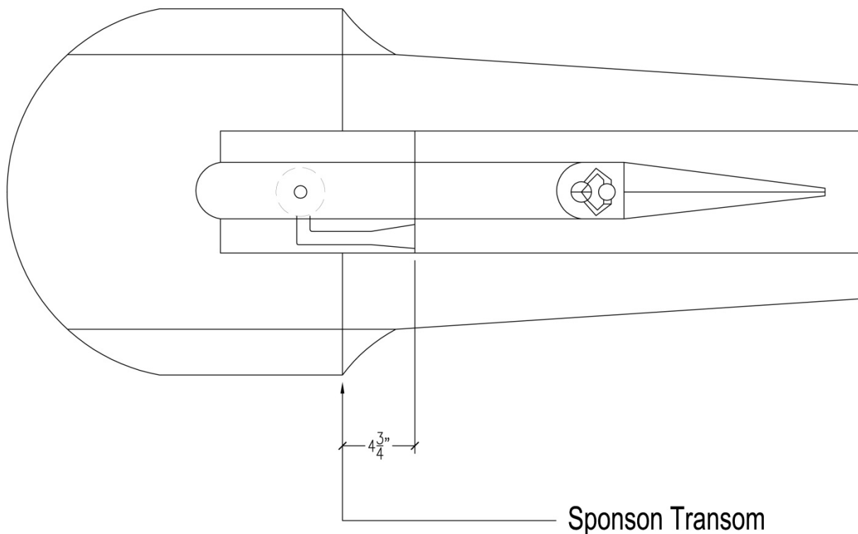
FIGURE 2 – Classic Thunderboat
