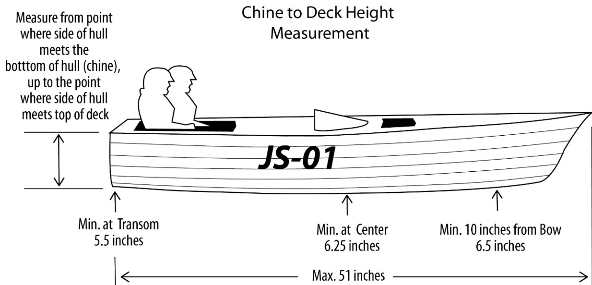
FIGURE 3 - Jersey Skiff
