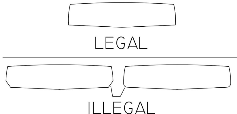
FIGURE - Crackerbox Hull
